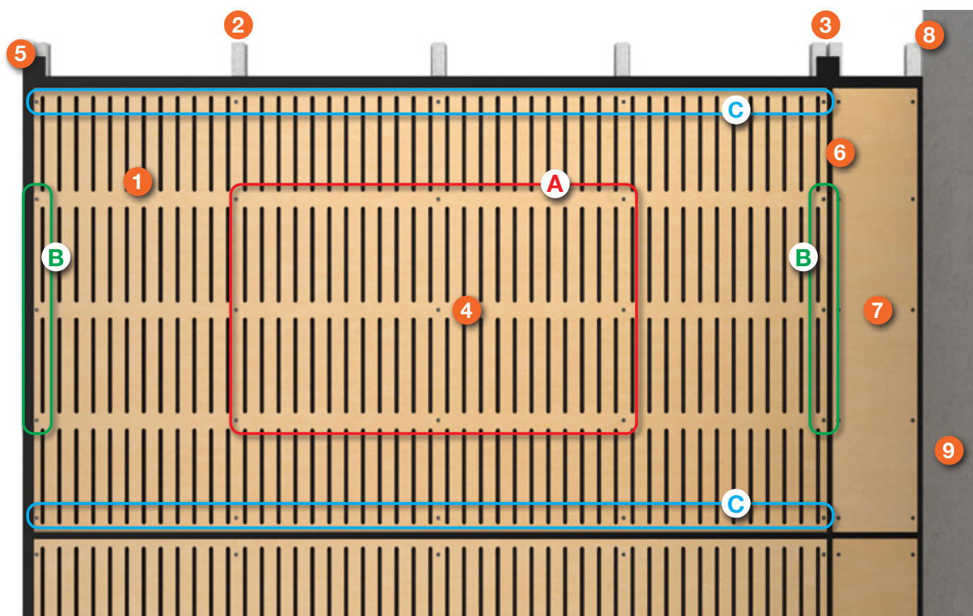
Figure 1: Typical face fix installation with 10mm expressed joint.
